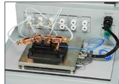
Hot plate shown integrated with Keysight Analyzer B1506A
